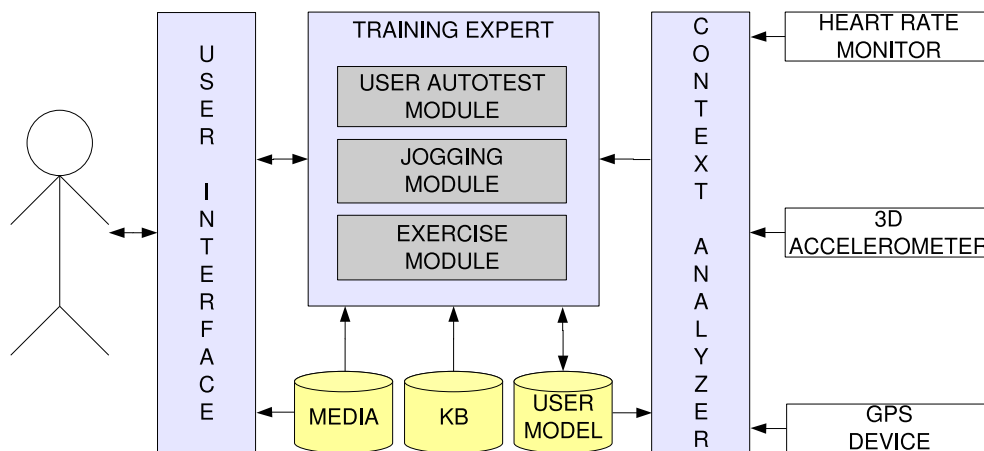
Fig. 5. MOPET architecture.
